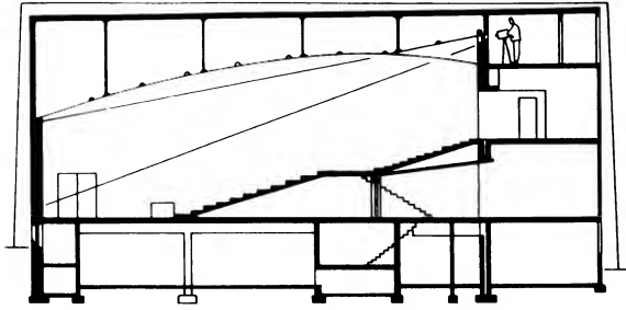
① Section → ②
